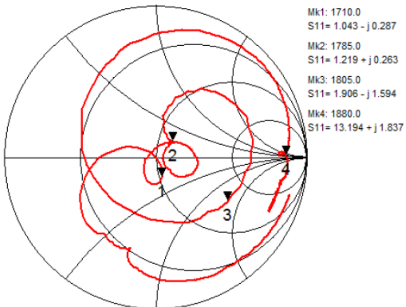
Smith Chart S11
