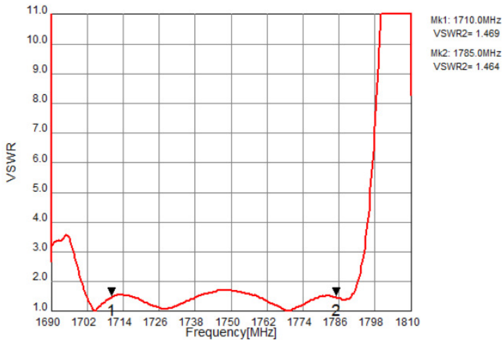
VSWR S22
