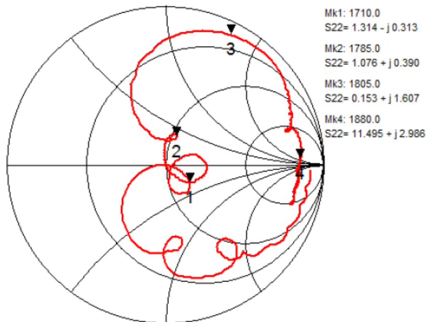
Smith Chart S22
